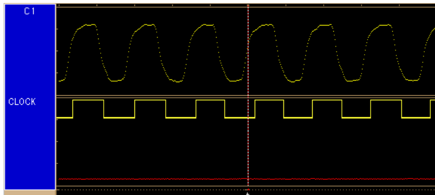
Figure 2.3 The same signal displayed by an oscilloscope and a timing analyzer
