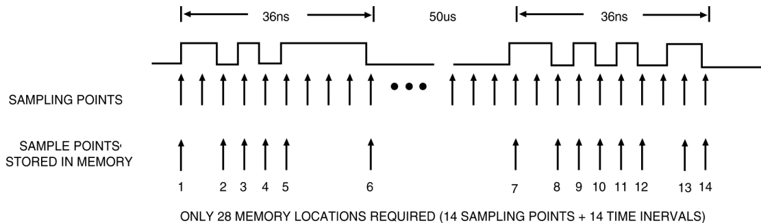
Figure 2.6 Sampling with a transition detector
