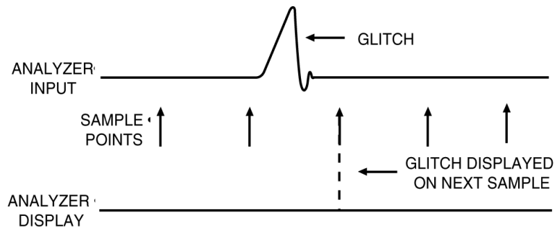
Figure 2.7 A glitch
