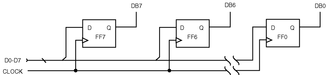
Figure 2.12 Eight D flip-flops in parallel connected to the same clock signal
