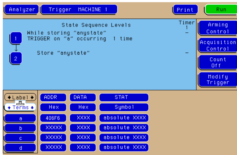
Figure 2.13 Trigger setup for the state analyzer
