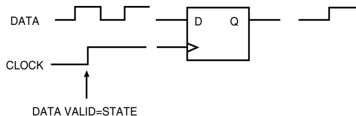
Figure 2.11 D flip-flop
