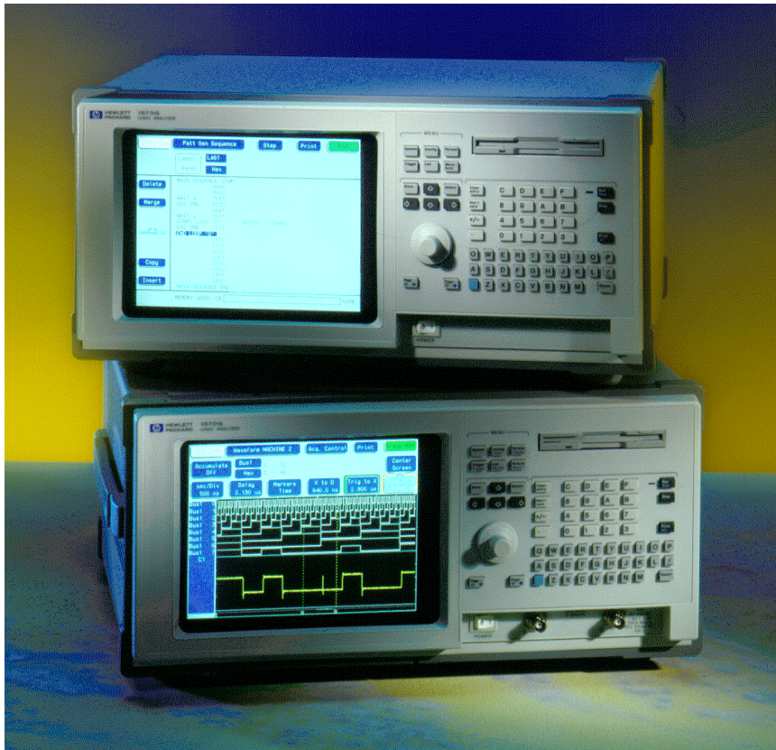
Figure 2.1 An analyzer with a built in pattern generator and an analyzer with a built in scope.
