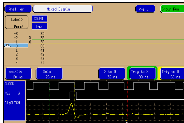
Figure 3.2 Cross-domain measurement
