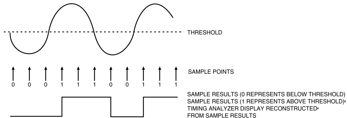
Figure 2.2 Timing analyzer sample points
