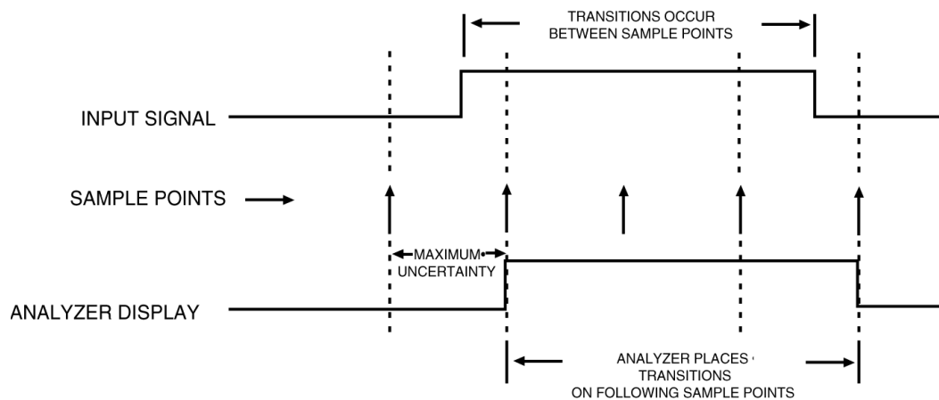
Figure 2.4 Timing analyzer sampling an input line
