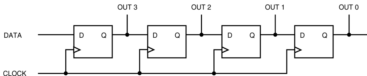
Figure 2.10 Edge-triggered shift register
