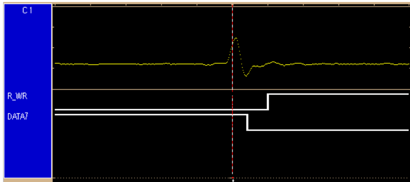
Figure 1.2 Oscilloscope and timing waveforms
