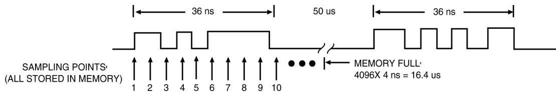
Figure 2.5 Sampling at high resolution
